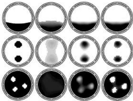
Figure 2 Visual evaluation of the reconstructed tomograms when using LBP thresholded, SIRT weighted, SIRT weighted and thresholded relative to the test reference for synthetic stratified, slug and bubble flows.
